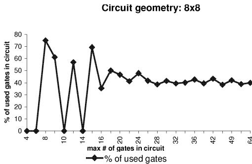
Fig. 5. Gate redundancy
